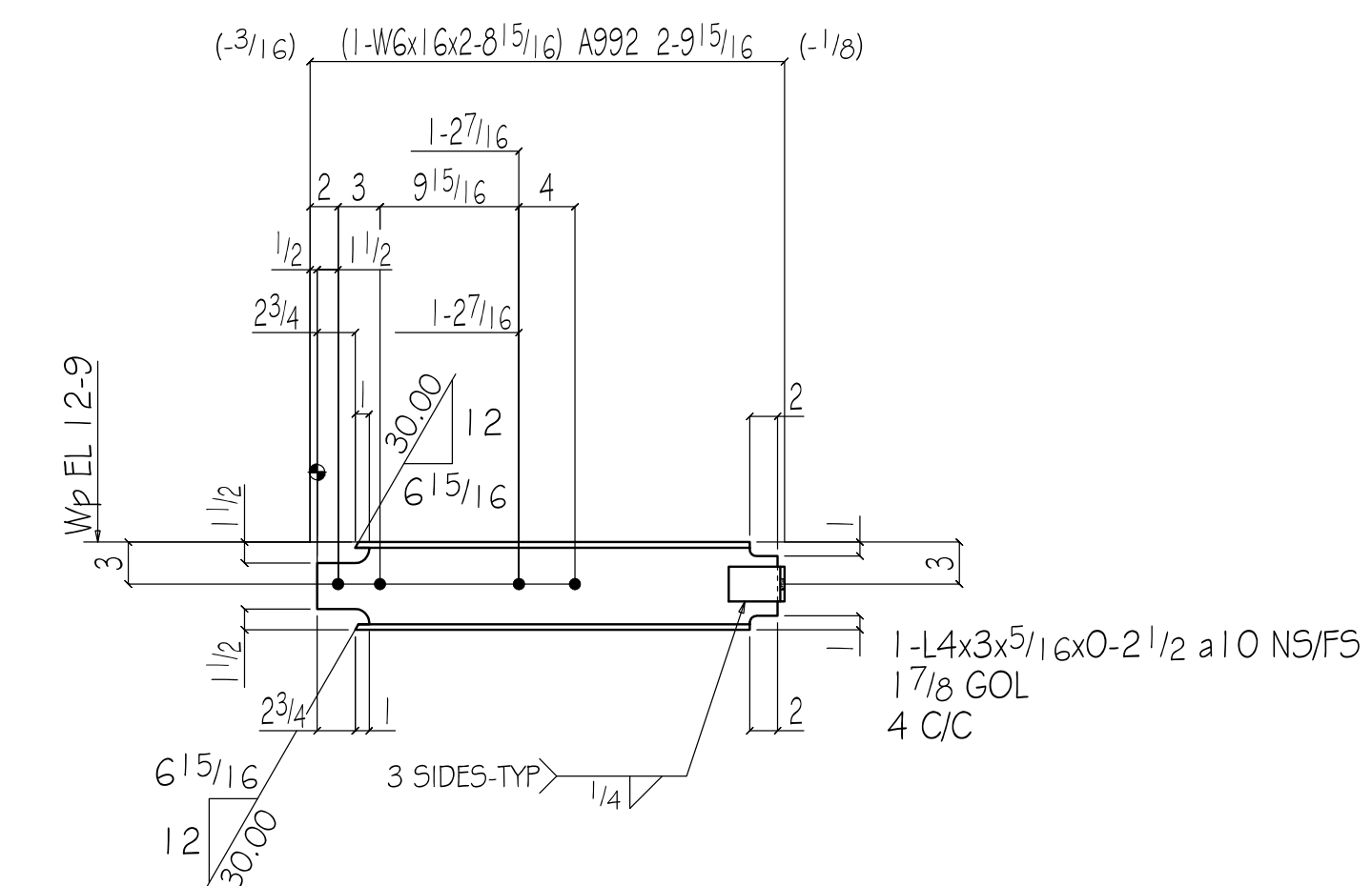
2 BEAMS 19B3
