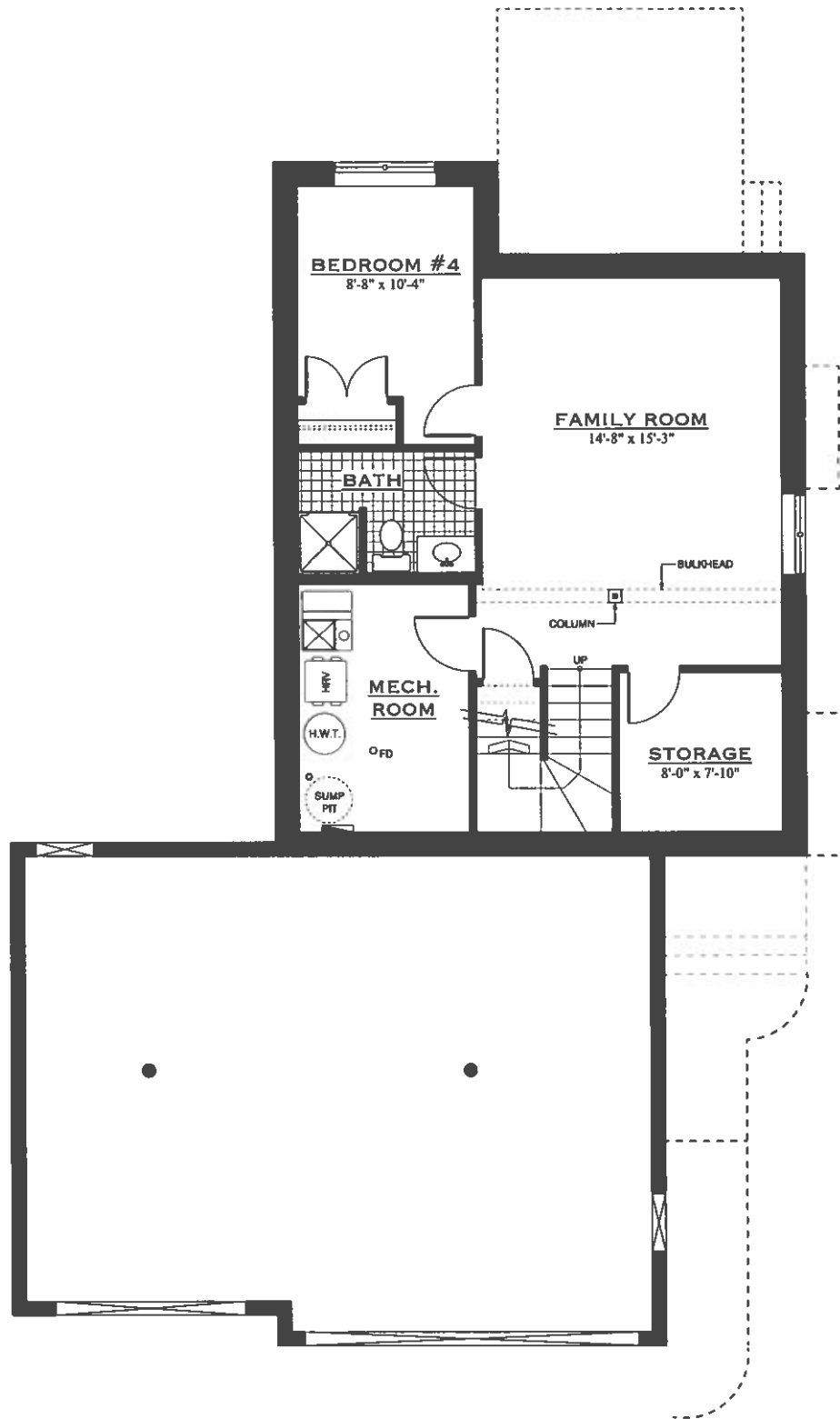
THE WELLINGTON BASEMENT PLAN 624 SQ. FT. (DEVELOPED)
