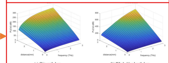
(a) Skin path loss (b) Whole blood path loss Fig. 3: Skin and whole blood path loss as function of distance and frequency.
