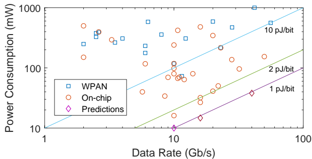
Figure 9: Energy efficiency of sub-THz and THz transceivers (from 0.06 to 0.43 THz) for short-range high-rate wireless applications.
