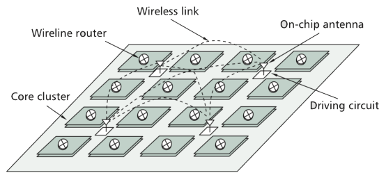
Figure 4: Envisioned high-level architecture for enabling on-chip communication [105]
