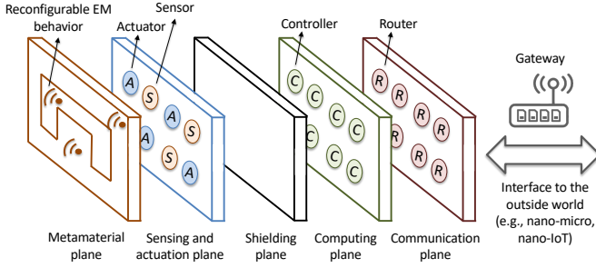
Figure 1: Envisioned high-level architecture for enabling software-defined metamaterials [72]
