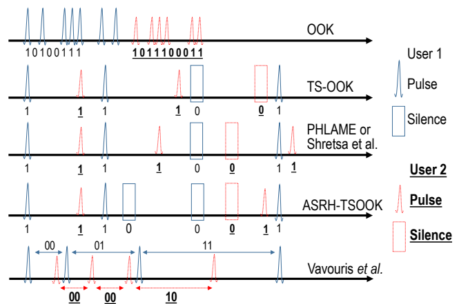
Figure 10: Comparison between the different variants of pulse-based OOK found in the literature [114], [165], [166], [168], [169].
