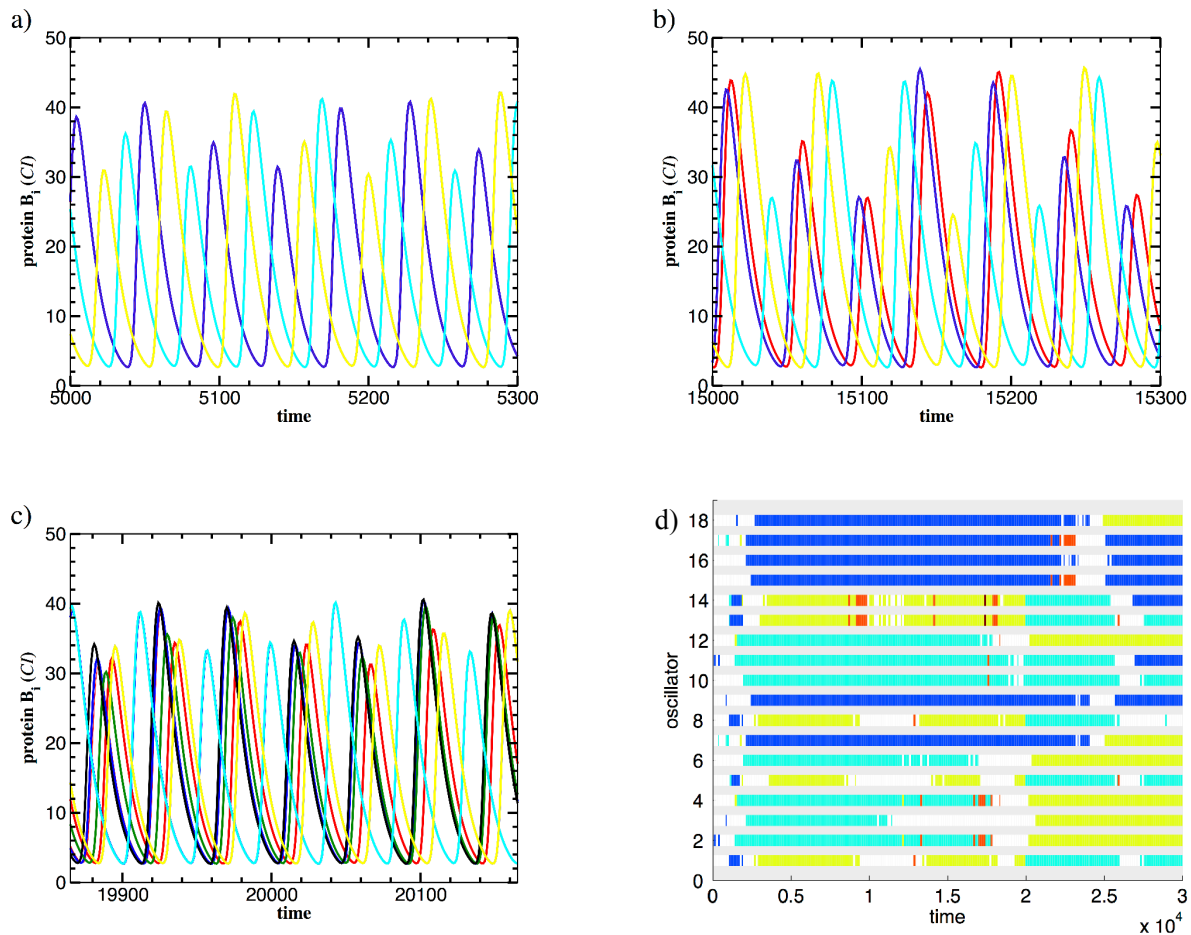
Figure 8. Chaotic behaviour seen in (a), (b), (c) time series of the same system of repressators taken at different time-points and (d) the corresponding cluster plot over the entire time span in the self-oscillatory regime of N = 18 oscillators with weak chaotic behaviour and long lasting grouping. The four figures have a matching colour coding.
