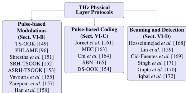
Figure 8: Classification of physical layer protocols for THz nanocommunication
