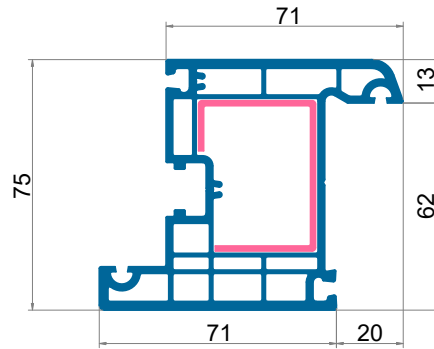
ESL 1804 Sash Profile
