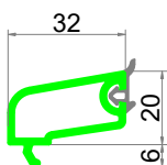
ESL 1808 24 mm Glazing Bead
