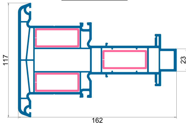
ESL 1813 In-Frame Mullion Profile
