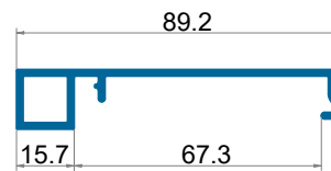
ESL 1818 Frame Channel Cover Profile
