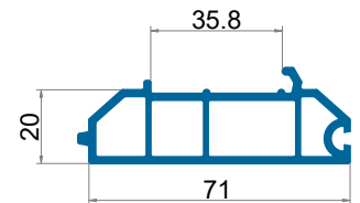
ESL 1826 Frame Threshold Cover Profile
