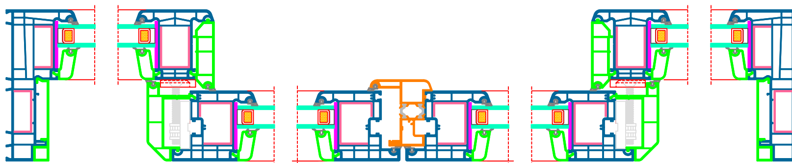
SECTION B-B
