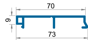
ESL 1828 Narrow Frame Channel Cover
