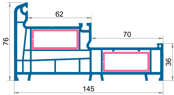
ESL 1802 Narrow Frame Profile
