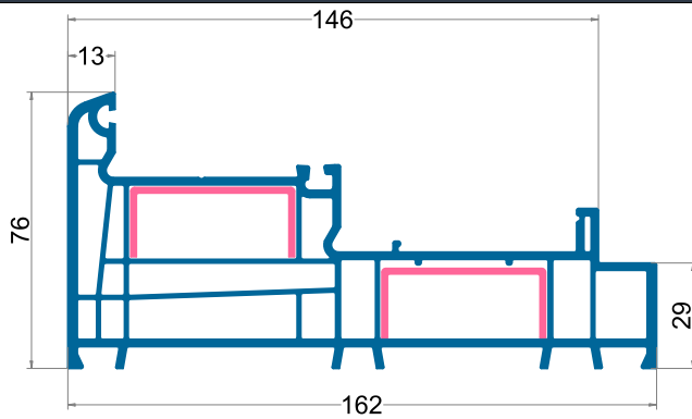
ESL 1801 Frame Profile
