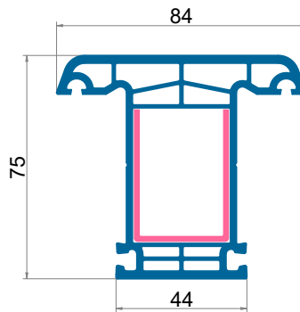
ESL 1803 Mullion Profile
