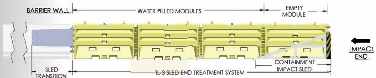
SLED™ TL-3 4900 lb. Pick-Up Truck Impact Attached to Concrete Median Barrier Wall
