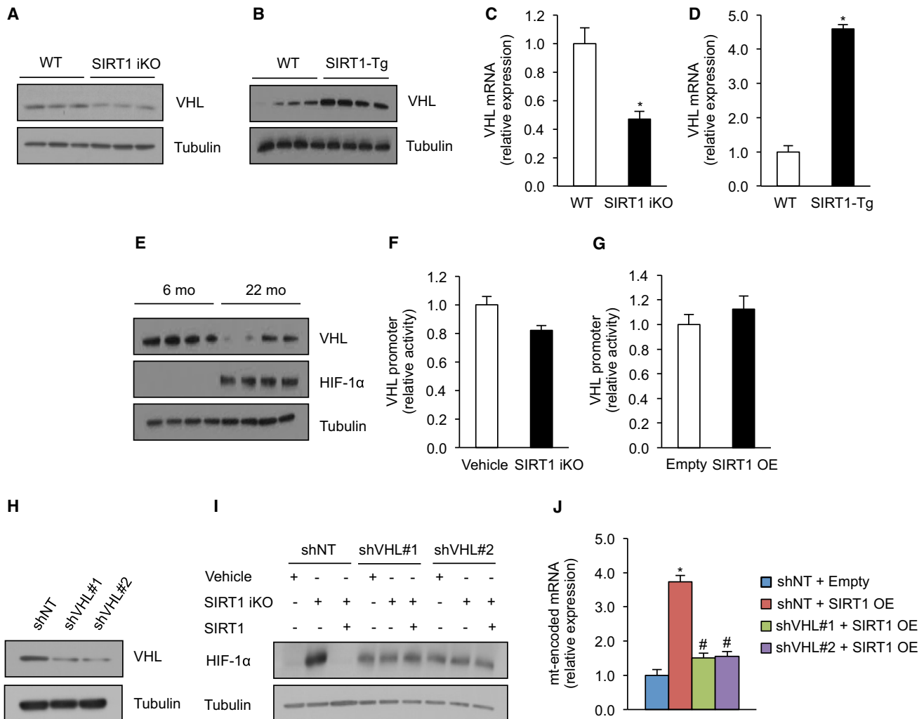
Figure 4. SIRT1 Regulates HIF-1 \alpha Stabilization in Skeletal Muscle through Regulation of VHL Expression
