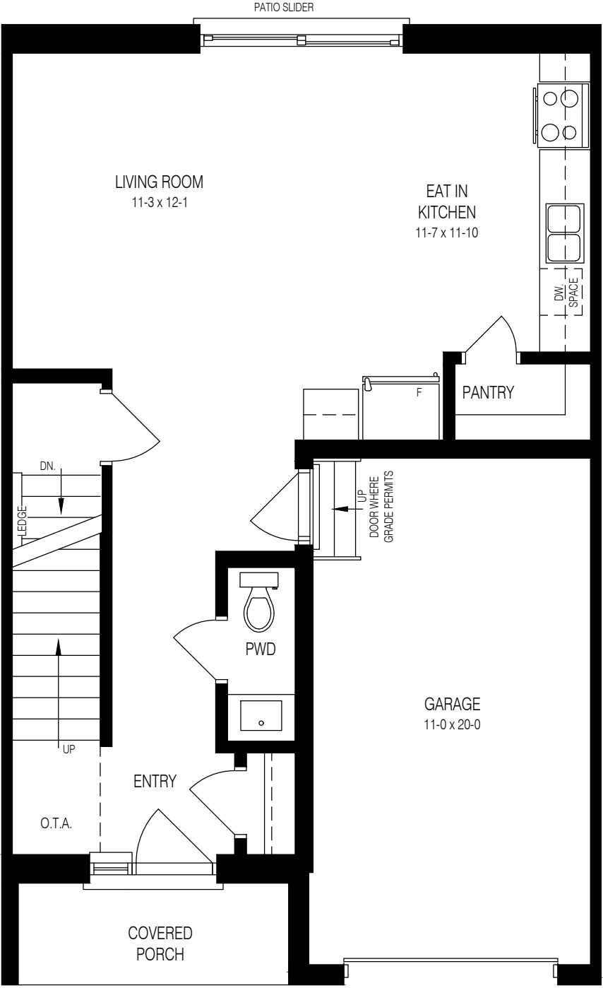
UNIT 3 - FARMHOUSE INTERIOR 'A' MAIN FLOOR PLAN
