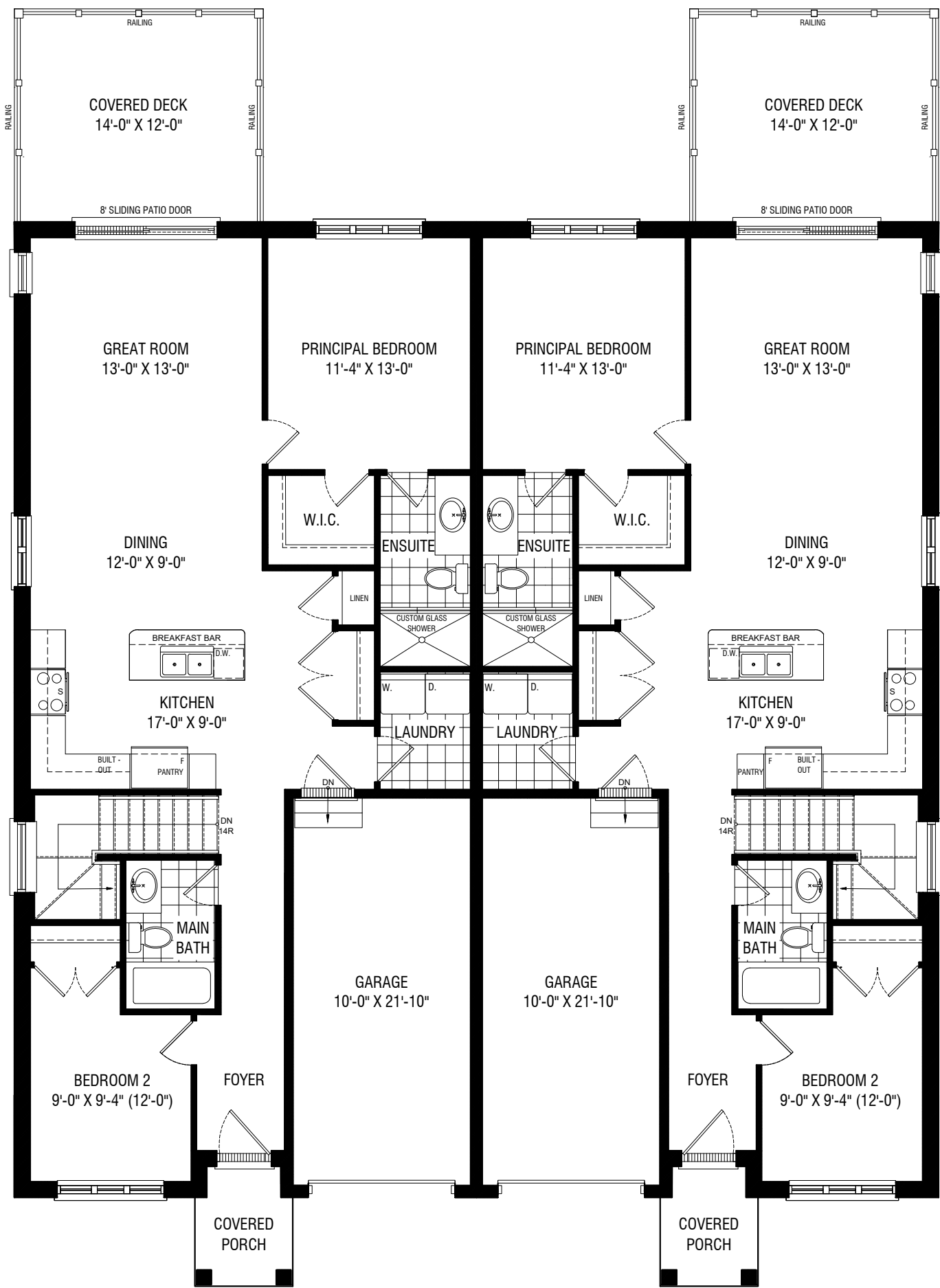
MAIN FLOOR PLAN A
