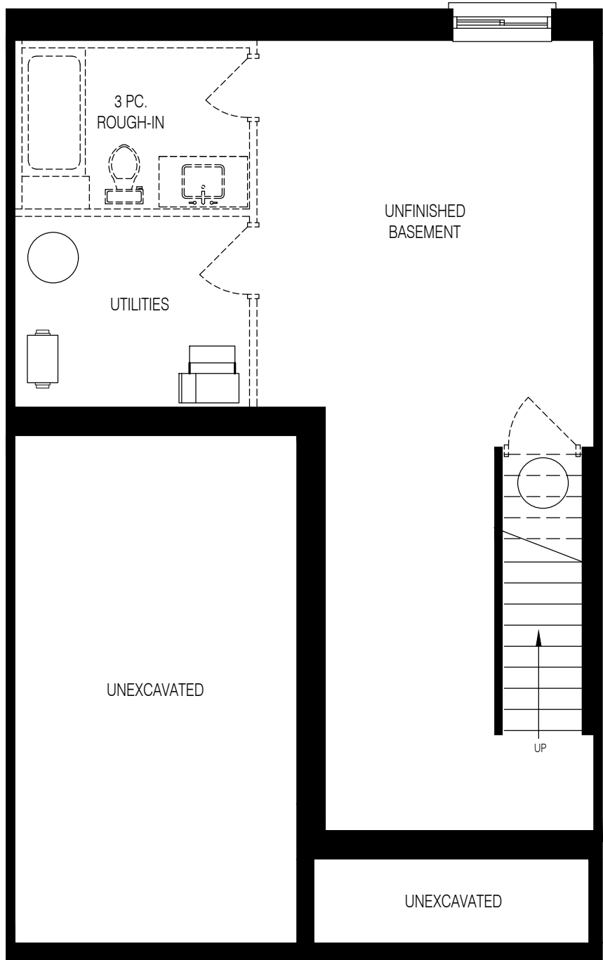
UNIT 2 AND 4- FARMHOUSE INTERIOR 'A' - MIRRORED BASEMENT FLOOR PLAN
