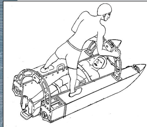
CPRA - Deployed, inflated, and in use
