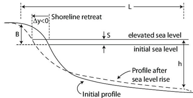
Figure 2: Bruun Rule of shoreline retreat
