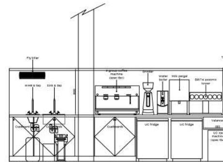
ELEVATION CC
