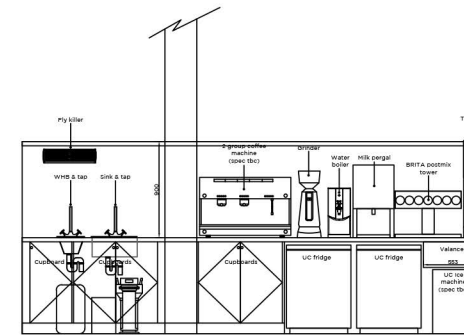
ELEVATION CC
