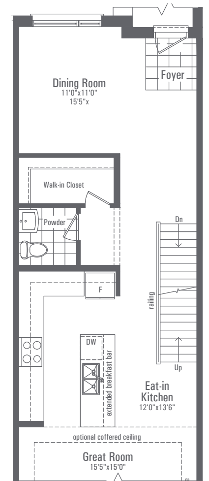
OPTIONAL KITCHEN LAYOUT
