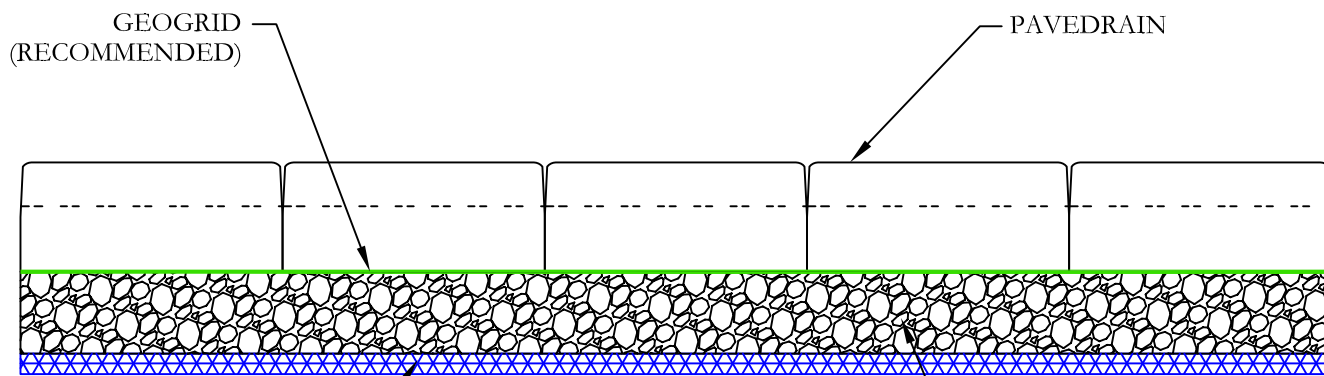
CROSS-SECTION SIDE VIEW
