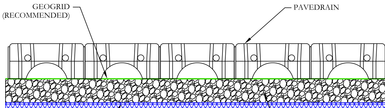
CROSS-SECTION END VIEW
