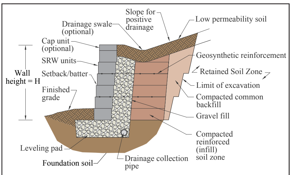
Figure 1—Reinforced Segmental Retaining Wall System Components
