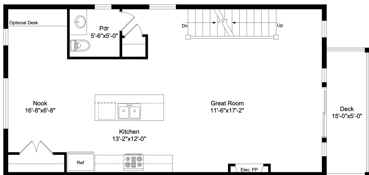
MAIN LEVEL FLOOR PLAN
