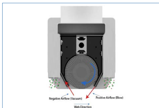
RoClean-C Web Cleaner (cross section of airflow and brush direction)
