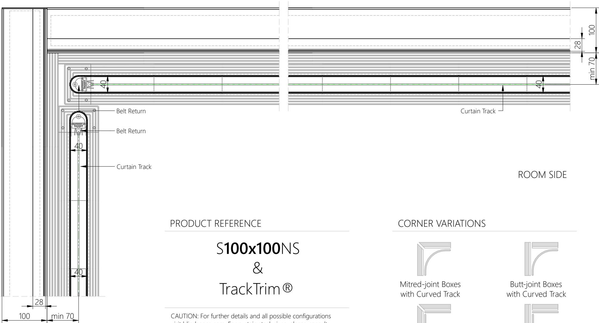
HEAD BOX S100x100NS & TRACKTRIM PROFILE
