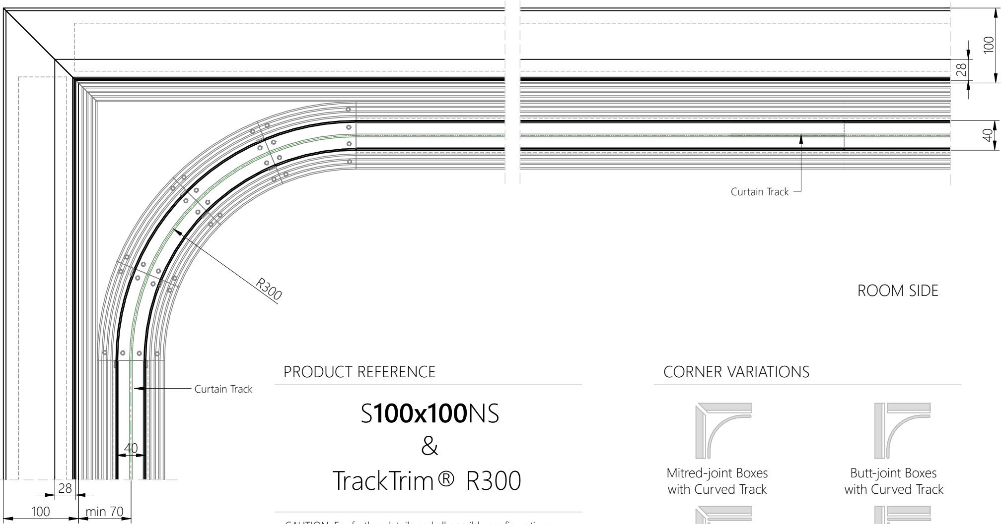
HEAD BOX S100x100NS & TRACKTRIM PROFILE
