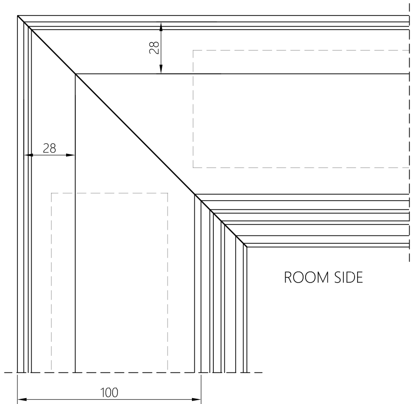
HEAD BOX S100X100NS
