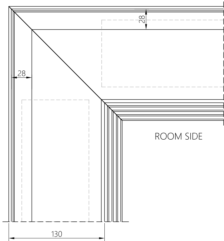
HEAD BOX S130X130NS
