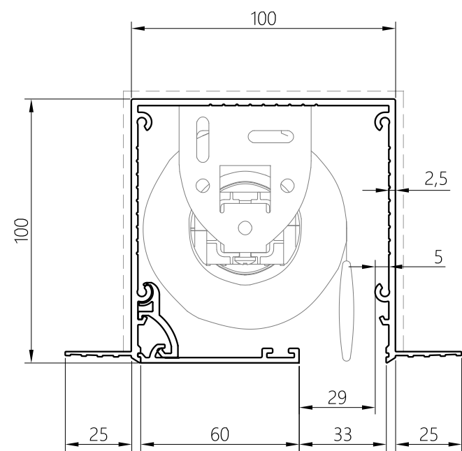
HEAD BOX S100x100SS
