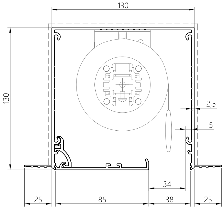
HEAD BOX S130x130SS
