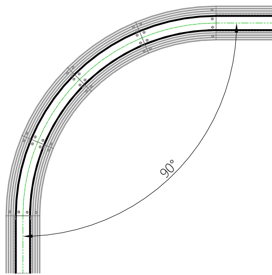
90° Turn using four TTCR508
