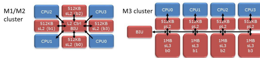
Figure 3. Comparison of M1/M2 with M3 CPU/cluster organization.
