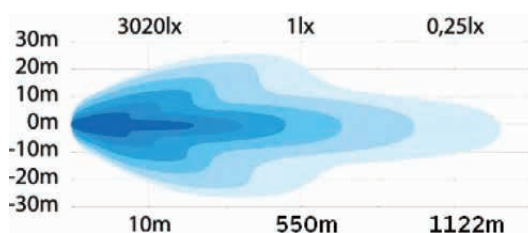
DRIVING LIGHT PATTERN
