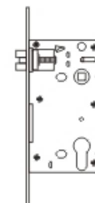
72x55 Lock Body
