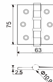
MSK 003 BEARING HINGE
