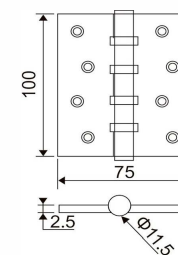
MSK 002 BEARING HINGE
