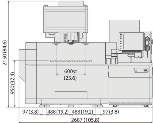
MV2400-R Layout Drawing
