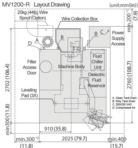
MV1200-R Layout Drawing
