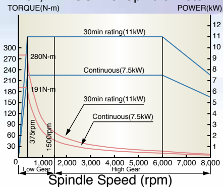
#40, 8,000rpm Spindle ZF Gear Box, FANUC \alpha 8i Spindle Motor
