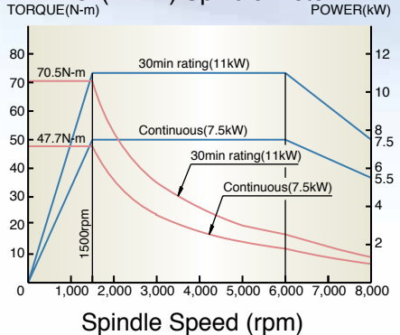
#40, 8,000rpm Spindle FANUC \alpha 8i (11kW) Spindle Motor
