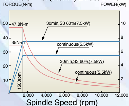
Directly coupled 12,000rpm FANUC \alpha 6i (7.5kW) Direct Drive
