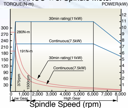
8,000rpm with ZF Gear Box FANUC \alpha 8i Spindle Motor
