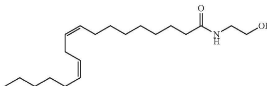
O-2050 (CAS: 667419-91-2)
