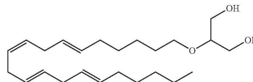
Anandamide (CAS: 94421-68-8)
