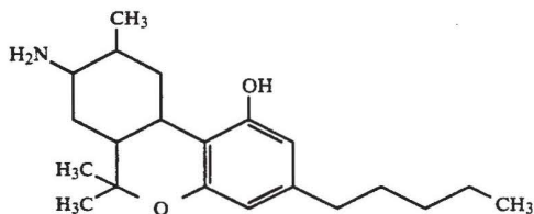
6aR-Trans-1-(hydroxy)-8-amino-6a,7,8,10,10a-hexahydro-6,6,9-trimethyl-3-pentyl-6H-dibenzo(b,d)pyran.
