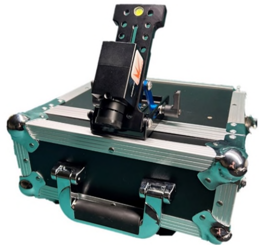
Truss Box w/ AIDA "Cube" camera & PROAIM mount
