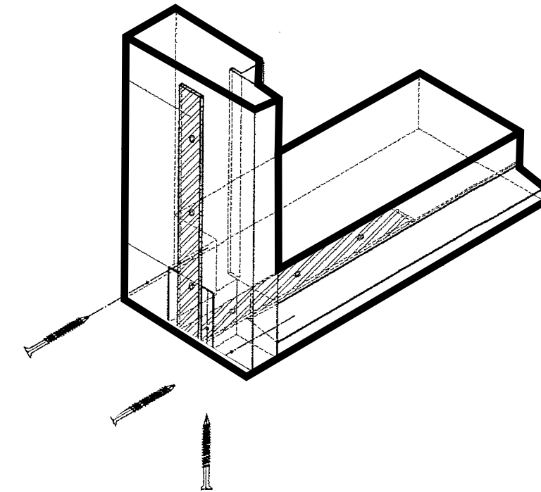
TYPICAL REGULAR FRAME BOTTOM CONNECTION
