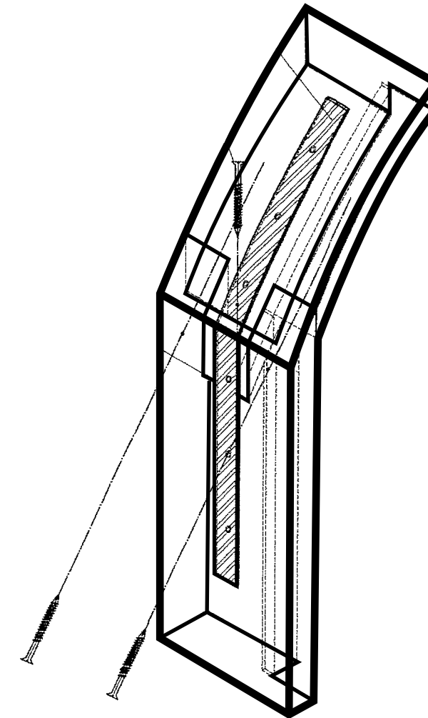
TYPICAL ARCHED / ELLIPTICAL FRAME TOP CONNECTION
