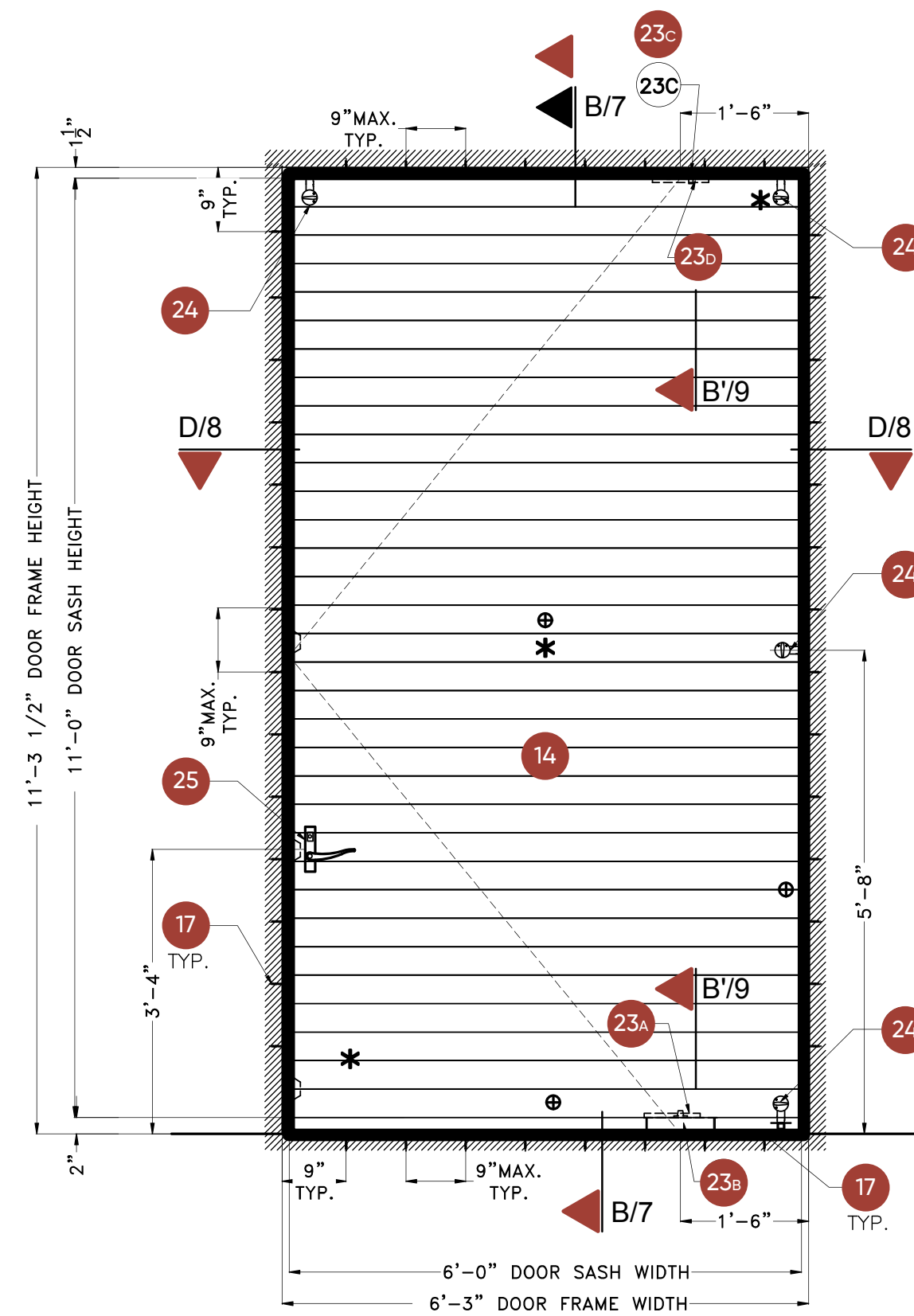
SPECIMEN #4: Exterior elevation (wood door)
