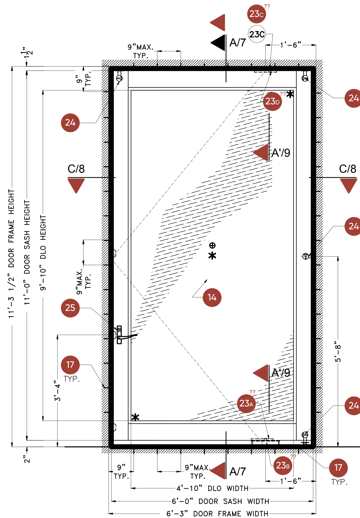
SPECIMEN #3: Exterior elevation (glass door)
