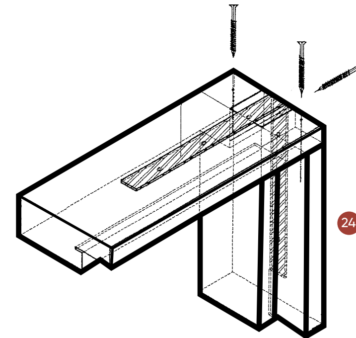
TYPICAL REGULAR FRAME TOP CONNECTION
