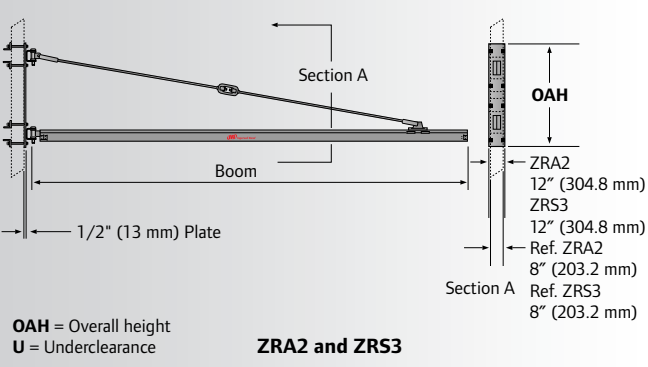
ZRA2 boom type wall mount (heavy)
