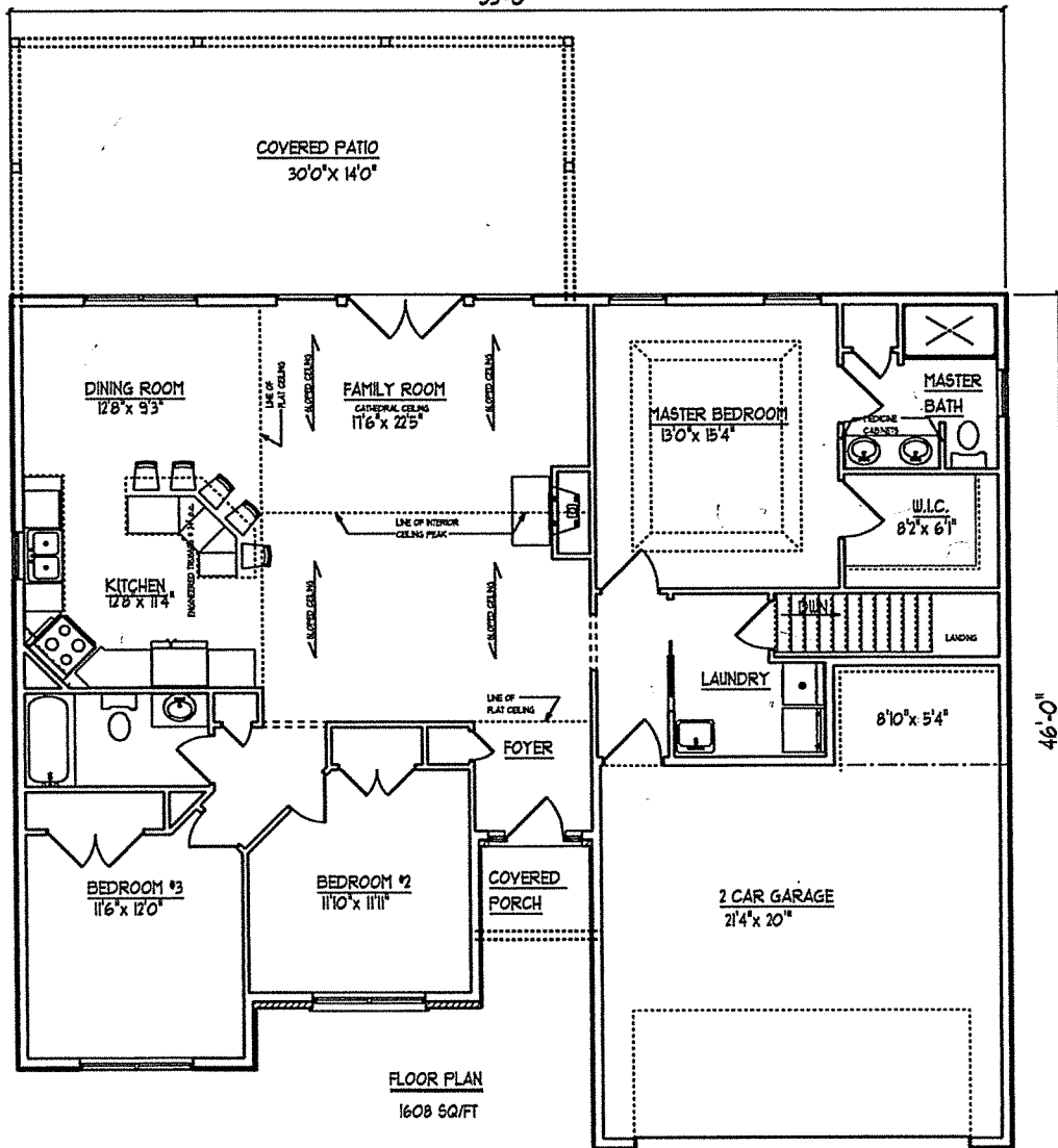
1608 SQ/FT RANCH 53'-0"
