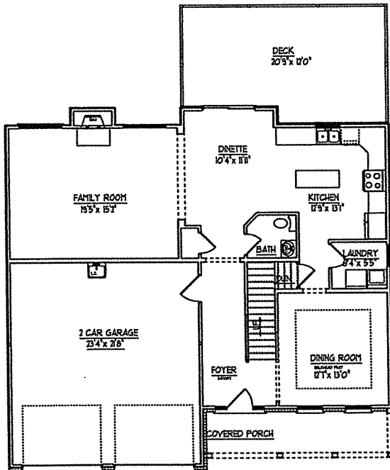
1ST FLOOR PLAN 1056 SQ/FT
