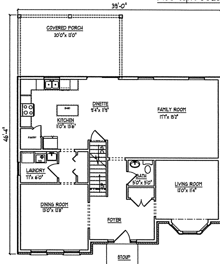
2450 sq/ft COLONIAL
