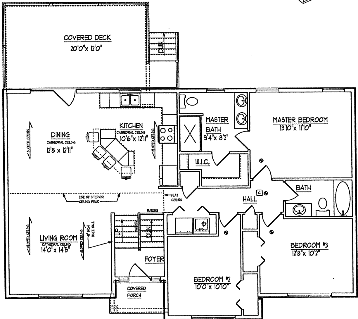
FLOOR PLAN 1400 SQ/FT
