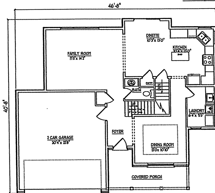
1ST FLOOR PLAN 934 sq/ft
