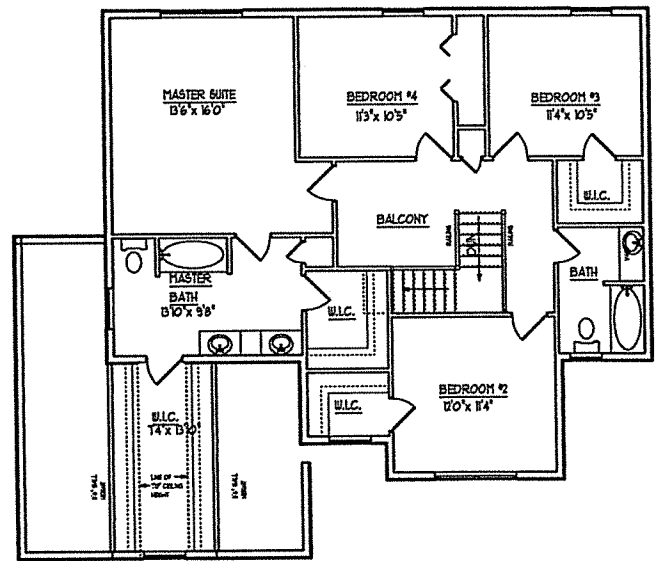
2ND FLOOR PLAN 1255 sq/ft
