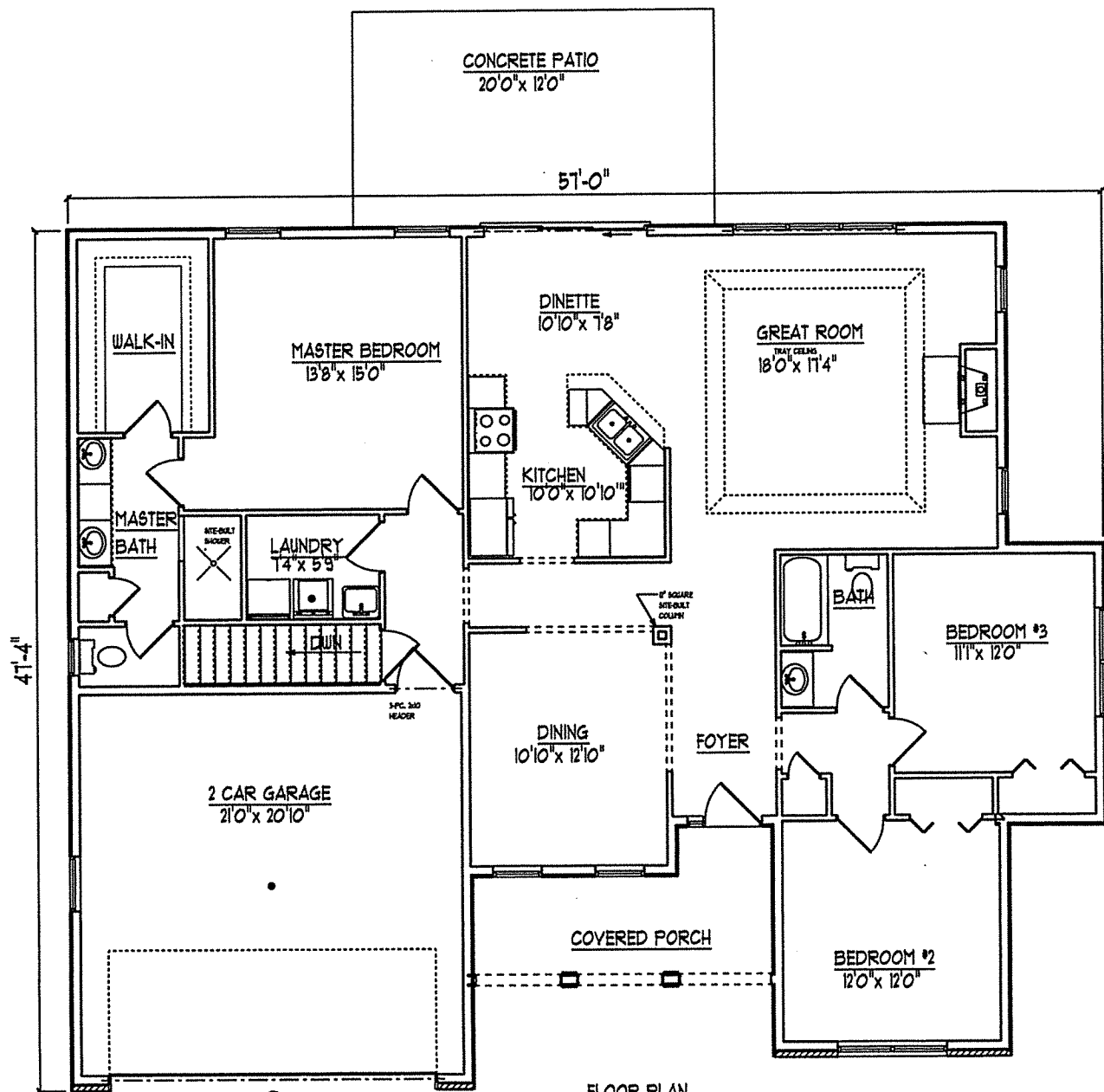
FLOOR PLAN 1110 SQ/FT
