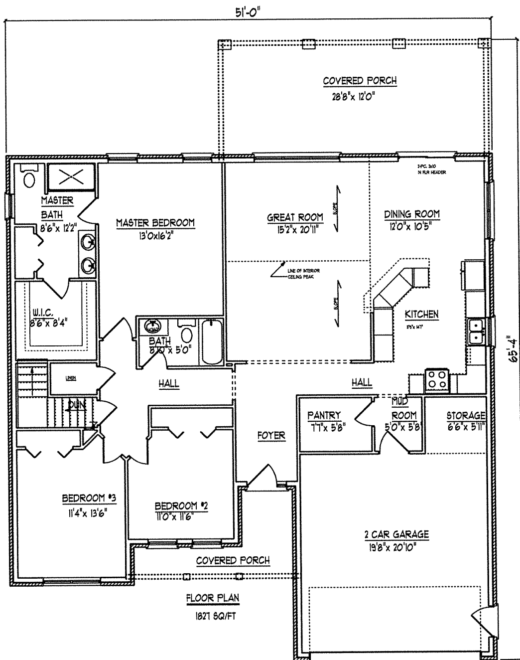
1827 SQ/FT RANCH
