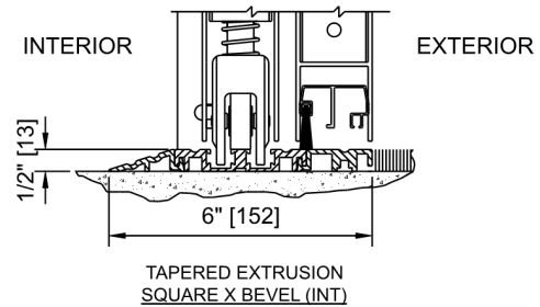
THRESHOLD -ONE SIDE TAPERED 4 1/2" FRAME
