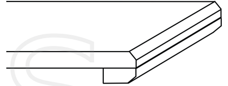
EP9 Laminated Bevel with bevelled strip
