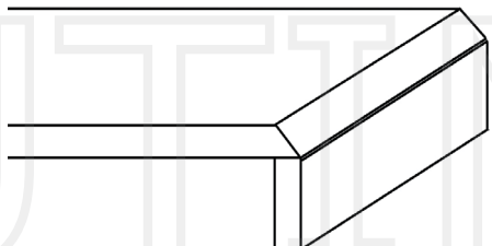
EP13 Laminated 45° Mitre with return strip
