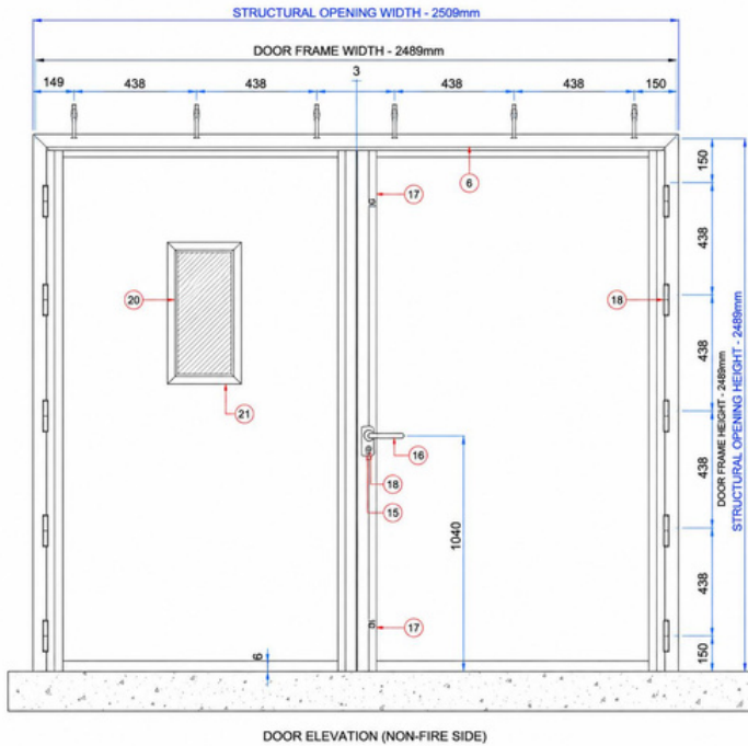
DOOR ELEVATION (NON-FIRE SIDE)
