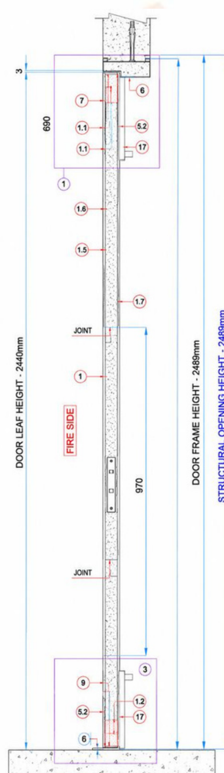
VERTICAL SECTION (SECTION B-B)
