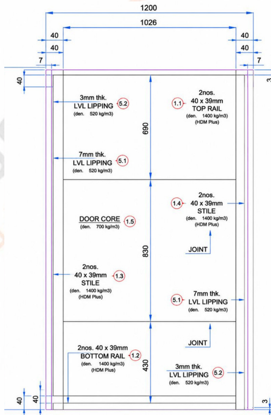
CORE CONSTRUCTION DETAILS (ACTIVE LEAF)
