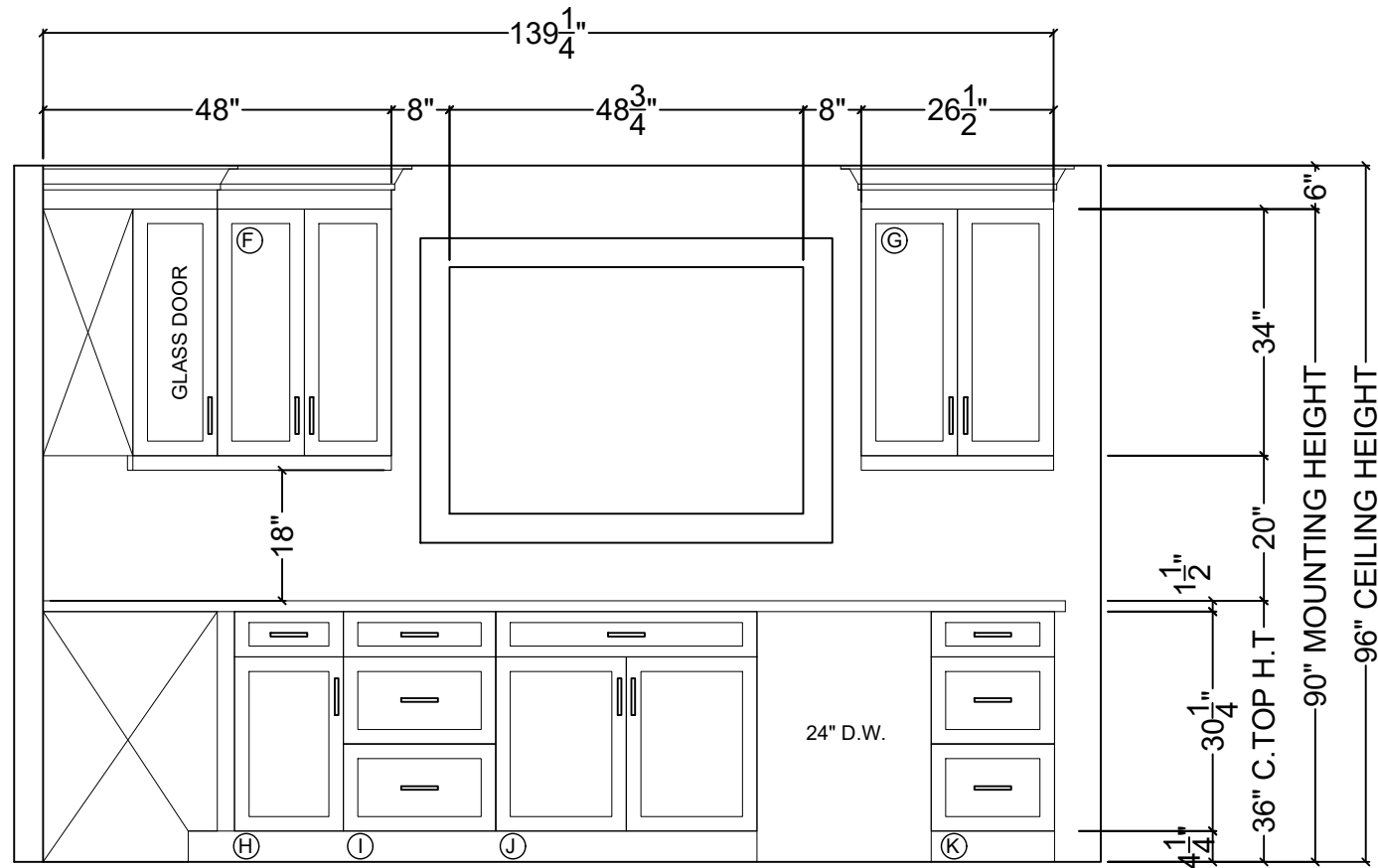
E2 KITCHEN ELEVATION
