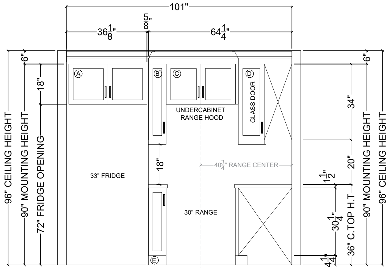
E1 KITCHEN ELEVATION
