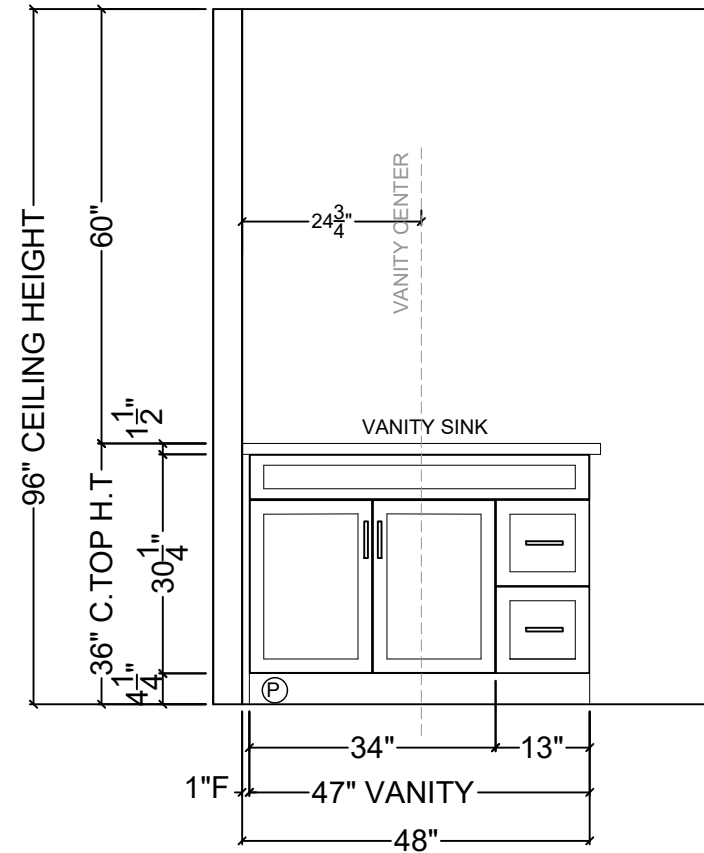
E6 MAIN BATH ELEVATION
