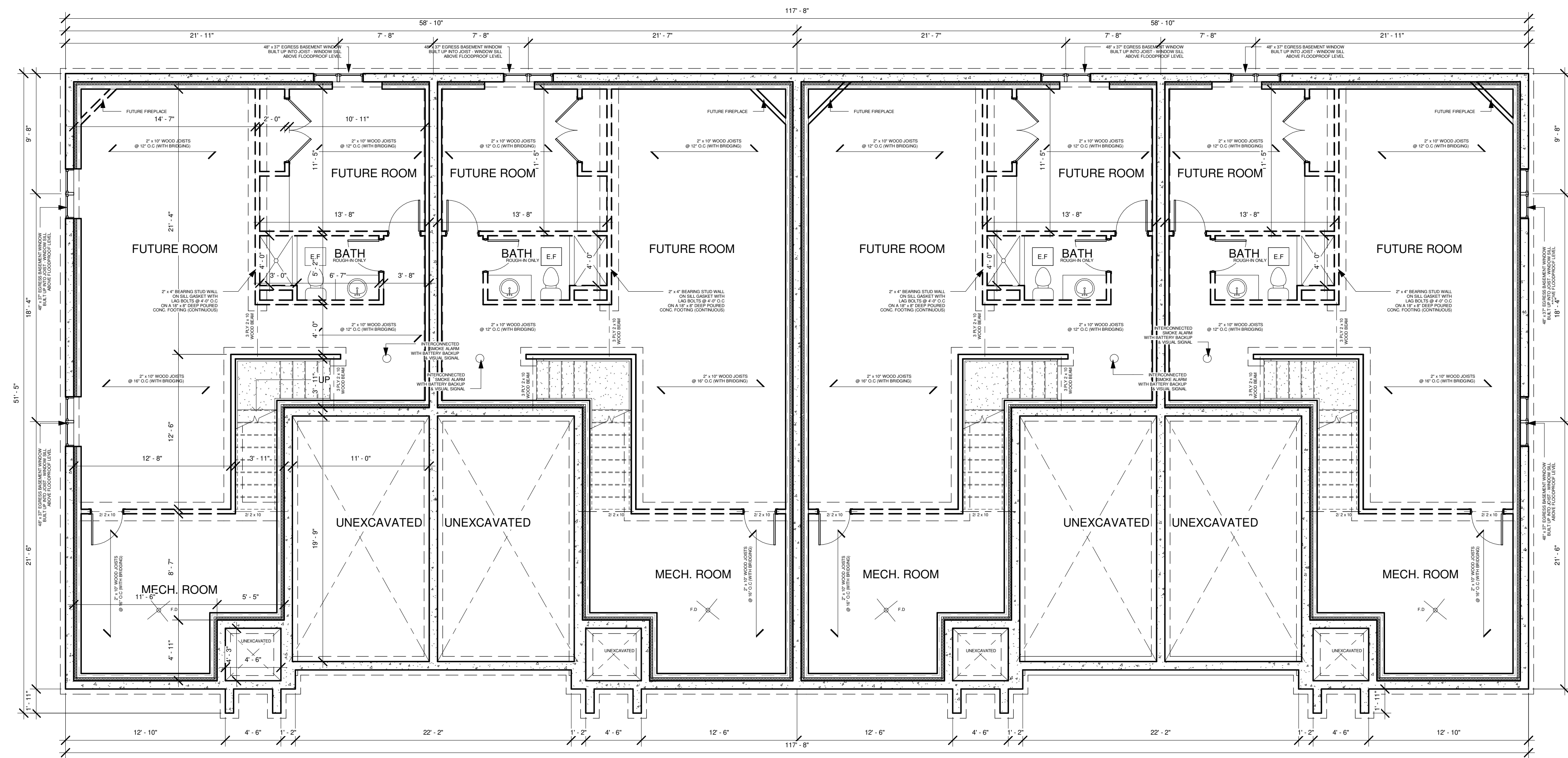
1 Basement 3/16" = 1'-0"
