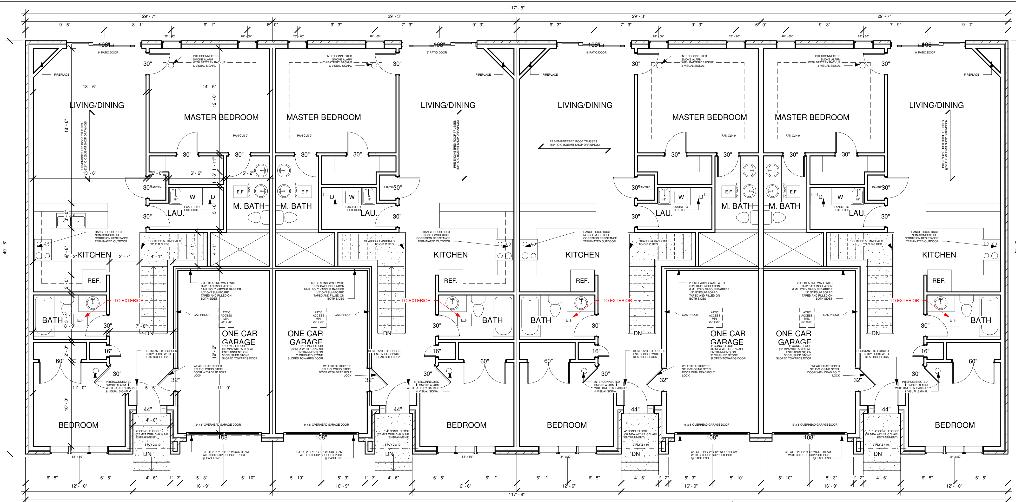
1 First Floor 3/16" = 1'-0"
