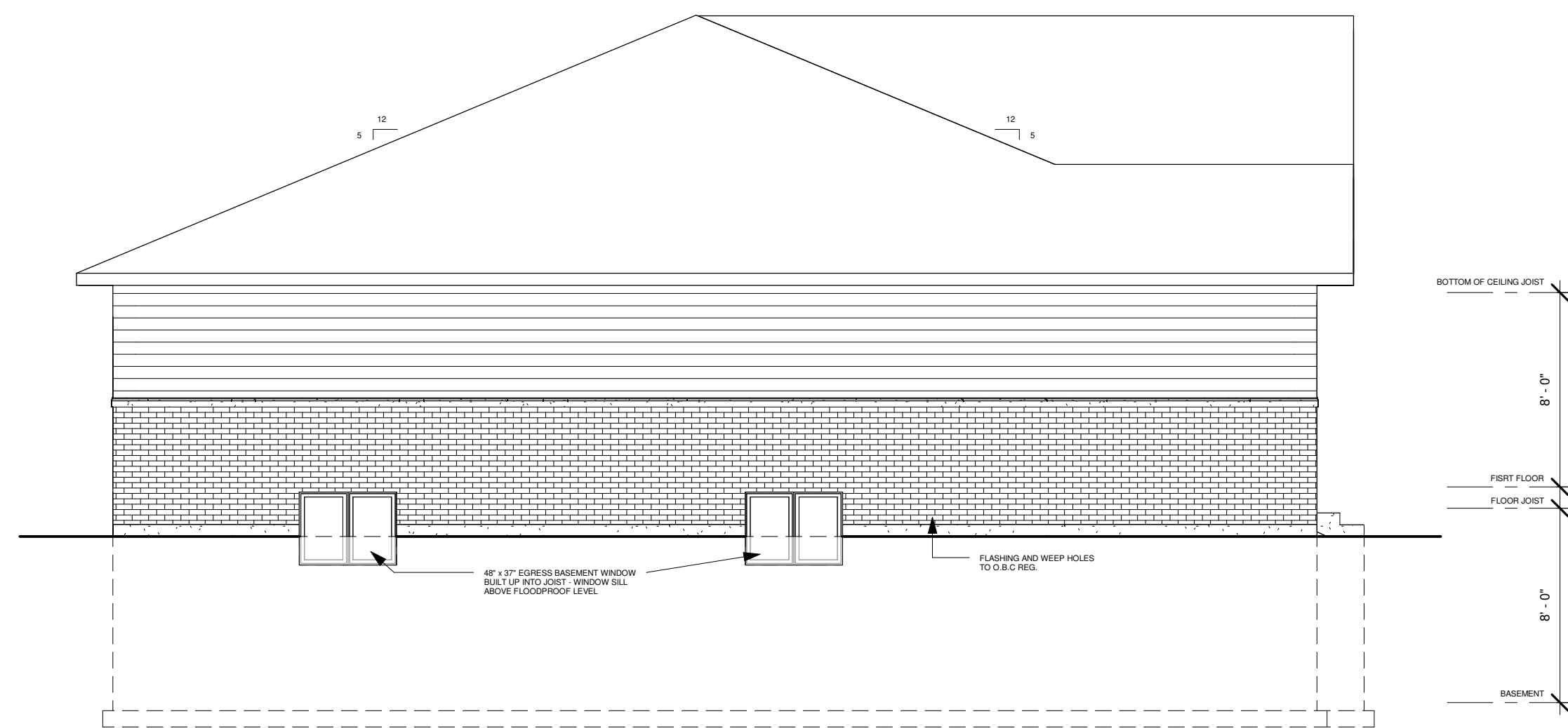
④ LEFT ELEVATION 3/16" = 1'-0"
