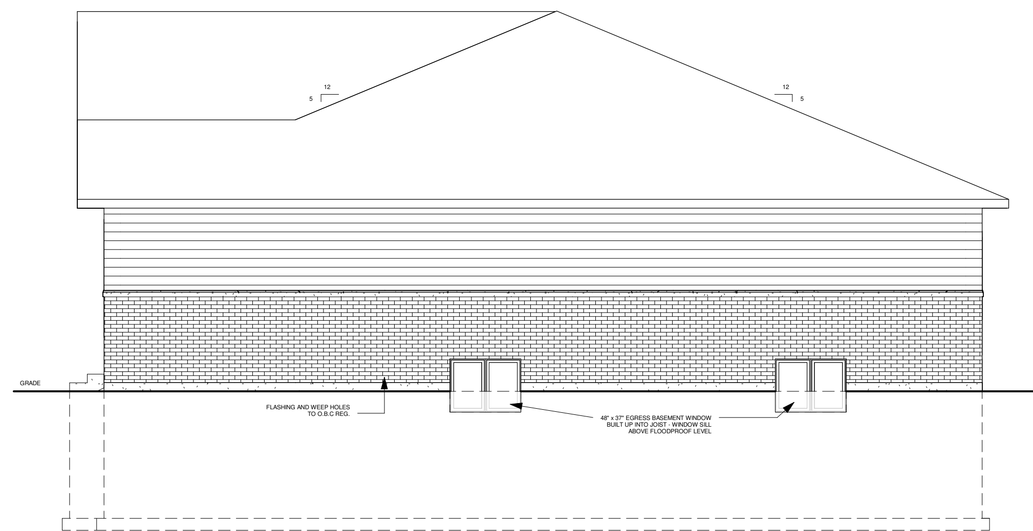
③ RIGHT ELEVATION 3/16" = 1'-0"
