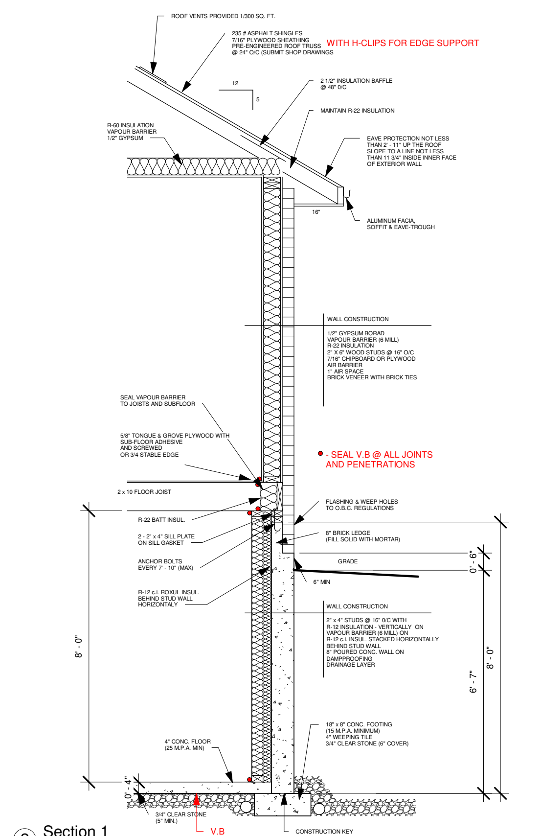
2 Section 1 3/8" = 1'-0"
