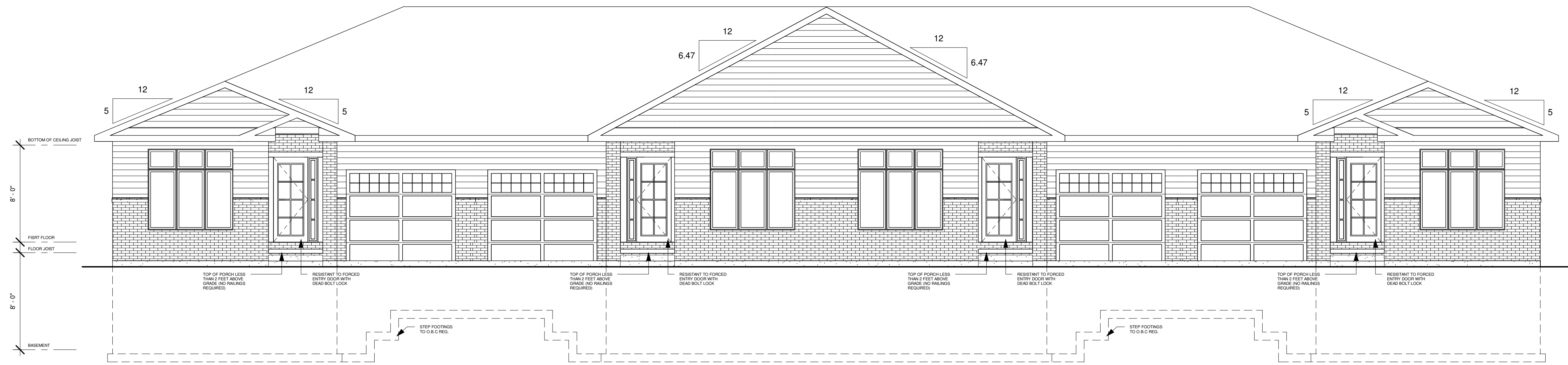
① FRONT ELEVATION 3/16" = 1'-0"
