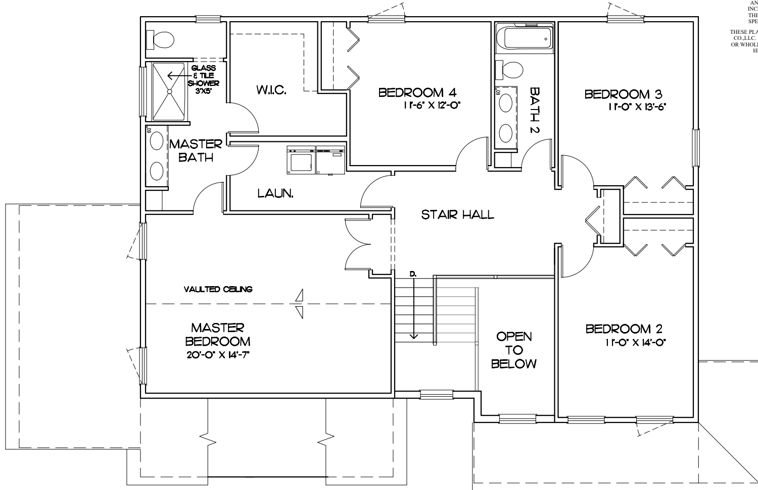
SECOND FLOOR PLAN / 8' CEILINGS
