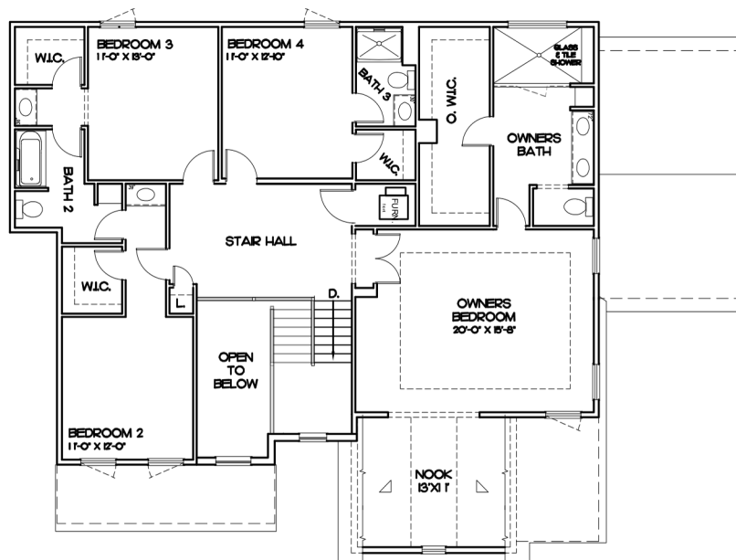
SECOND FLOOR PLAN / 9' CEILINGS
