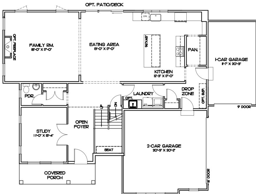
FIRST FLOOR PLAN / 9' CEILINGS
