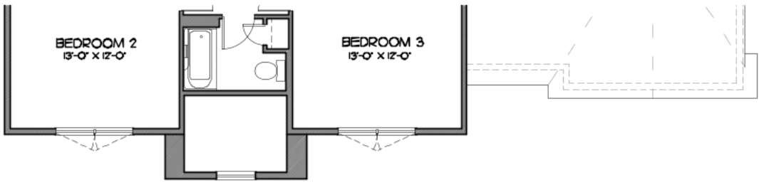
BRECKENRIDGE MANOR ELEVATION SECOND FLOOR PLAN | 9' WALLS
