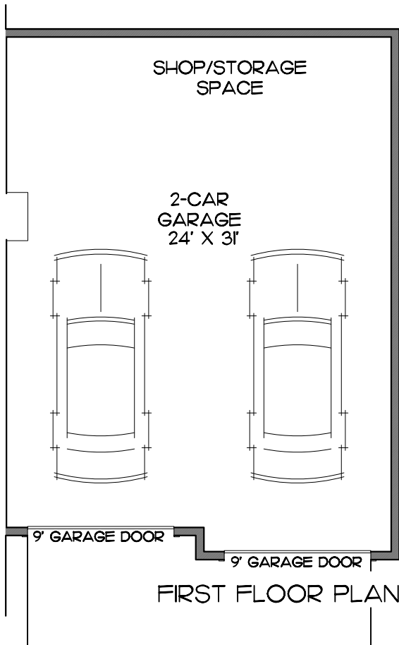
FOUNDATION PLAN
