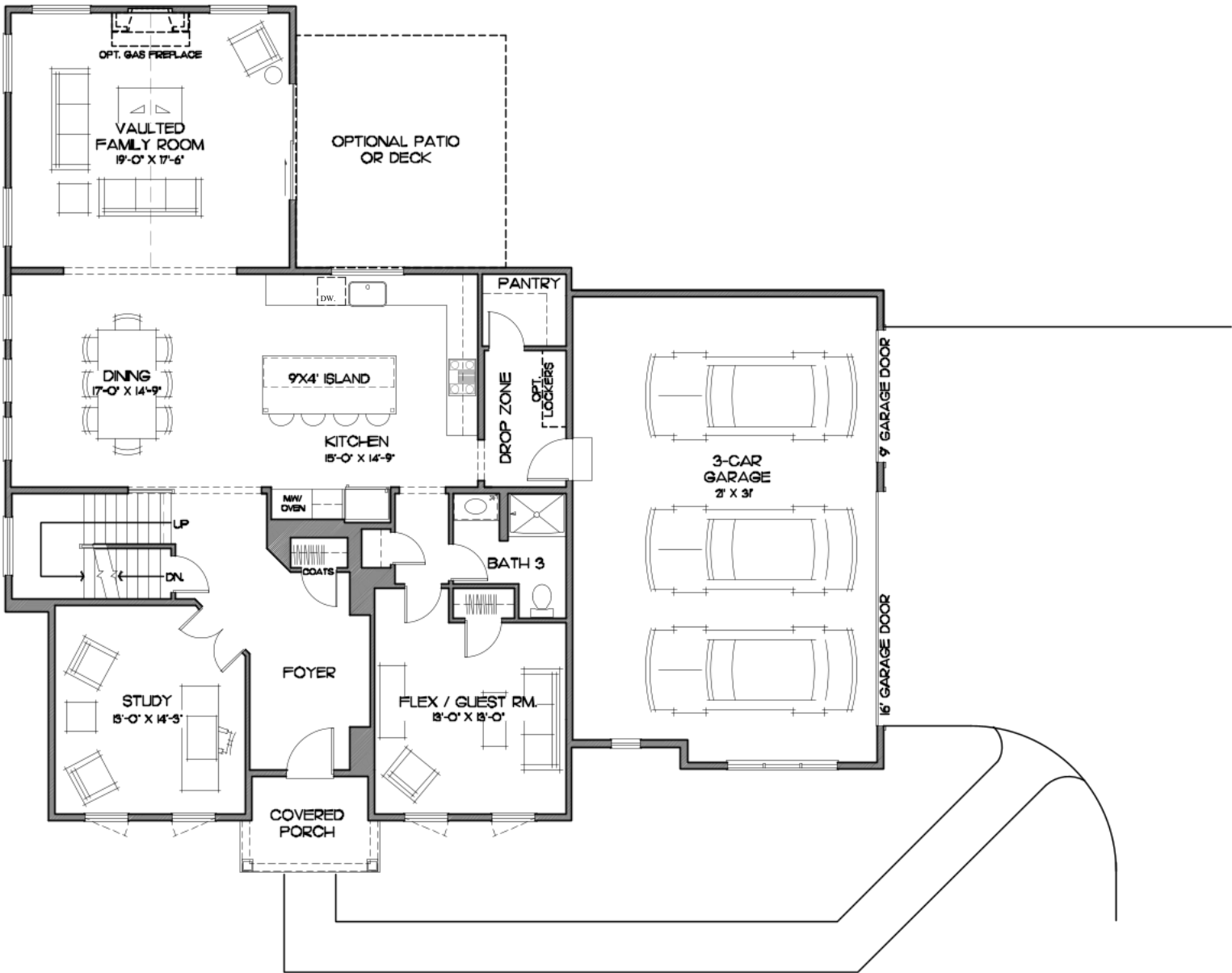
BRECKENRIDGE CLASSIC,& HOMESTEAD ELEVATION FIRST FLOOR PLAN | 10' WALLS
