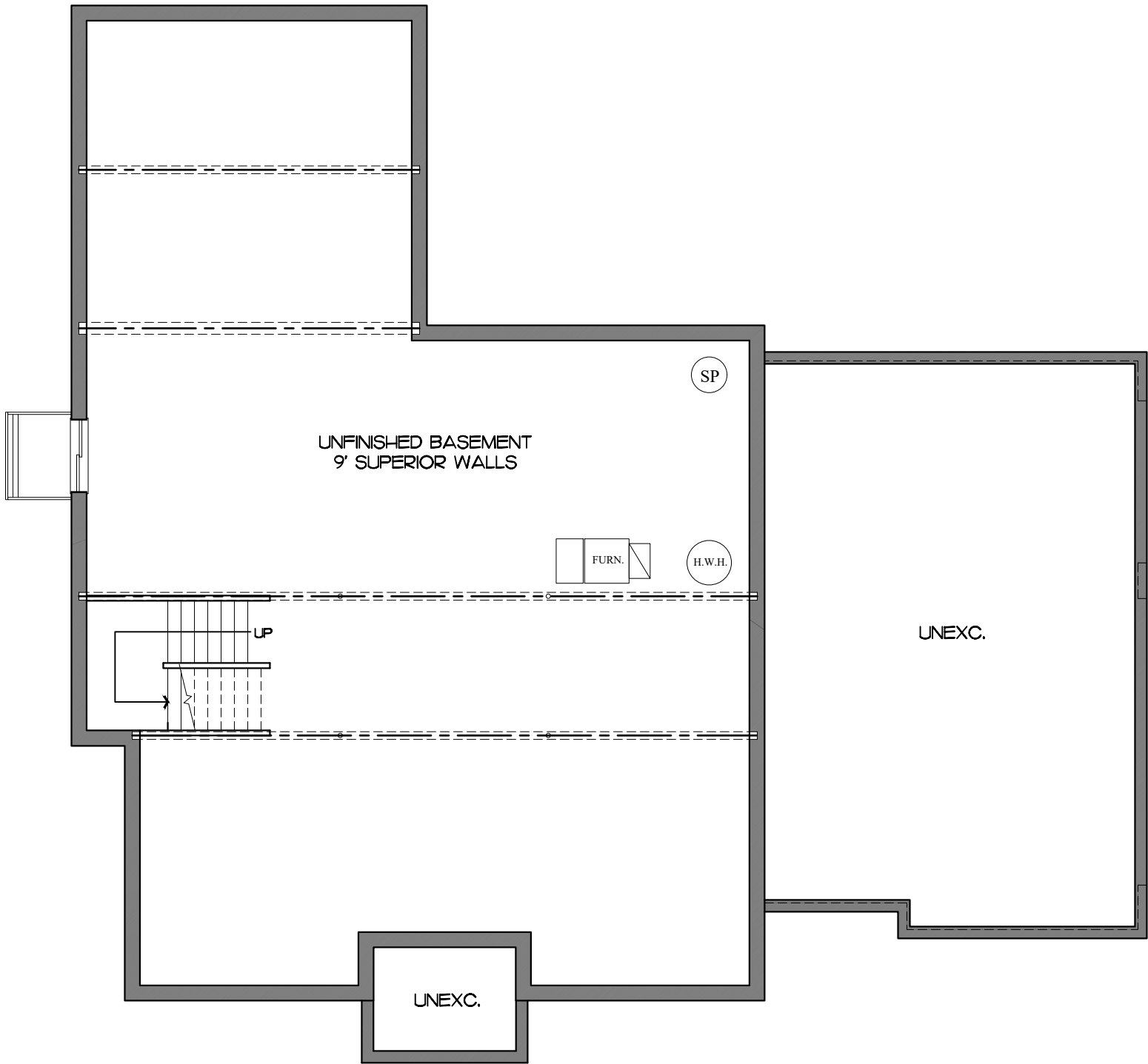
FOUNDATION PLAN
