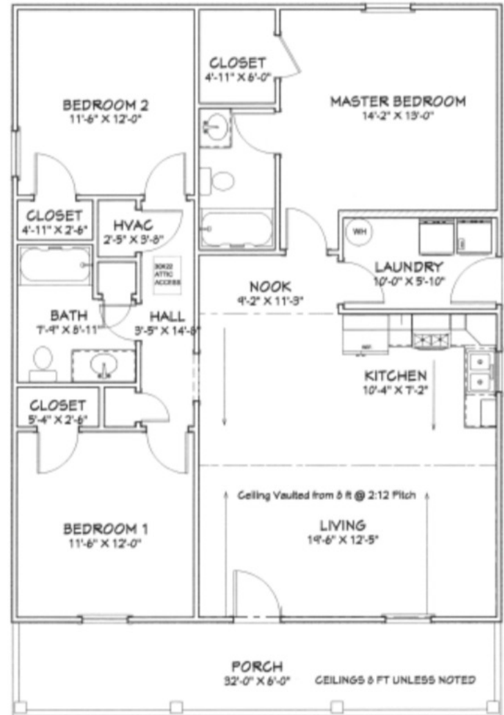
Floor Plan
